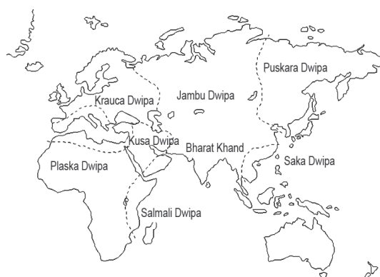
Figure 1.5 Seven Dvipas of the World as conceived in Ancient India
